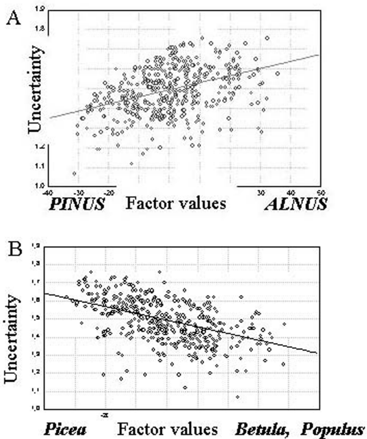
Fig. 2. Interpretation of uncertainty measures for trees and bush layers in relation to topography: A – factor of mineral nutrients supply, B – factor of recovery succession stage.
